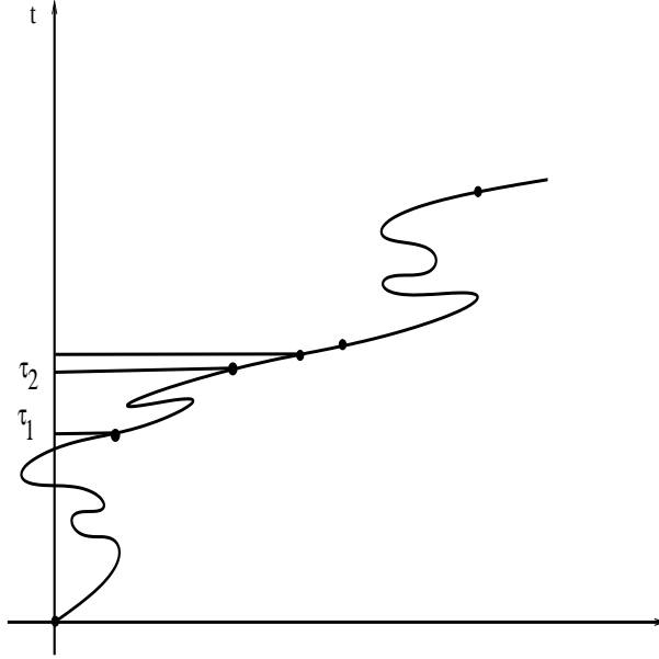
Figure 2: The projection of the path X_t \cdot \ell (horizontal axis) vs. time t (vertical axis), and the first two regeneration times \tau_1 and \tau_2 .
