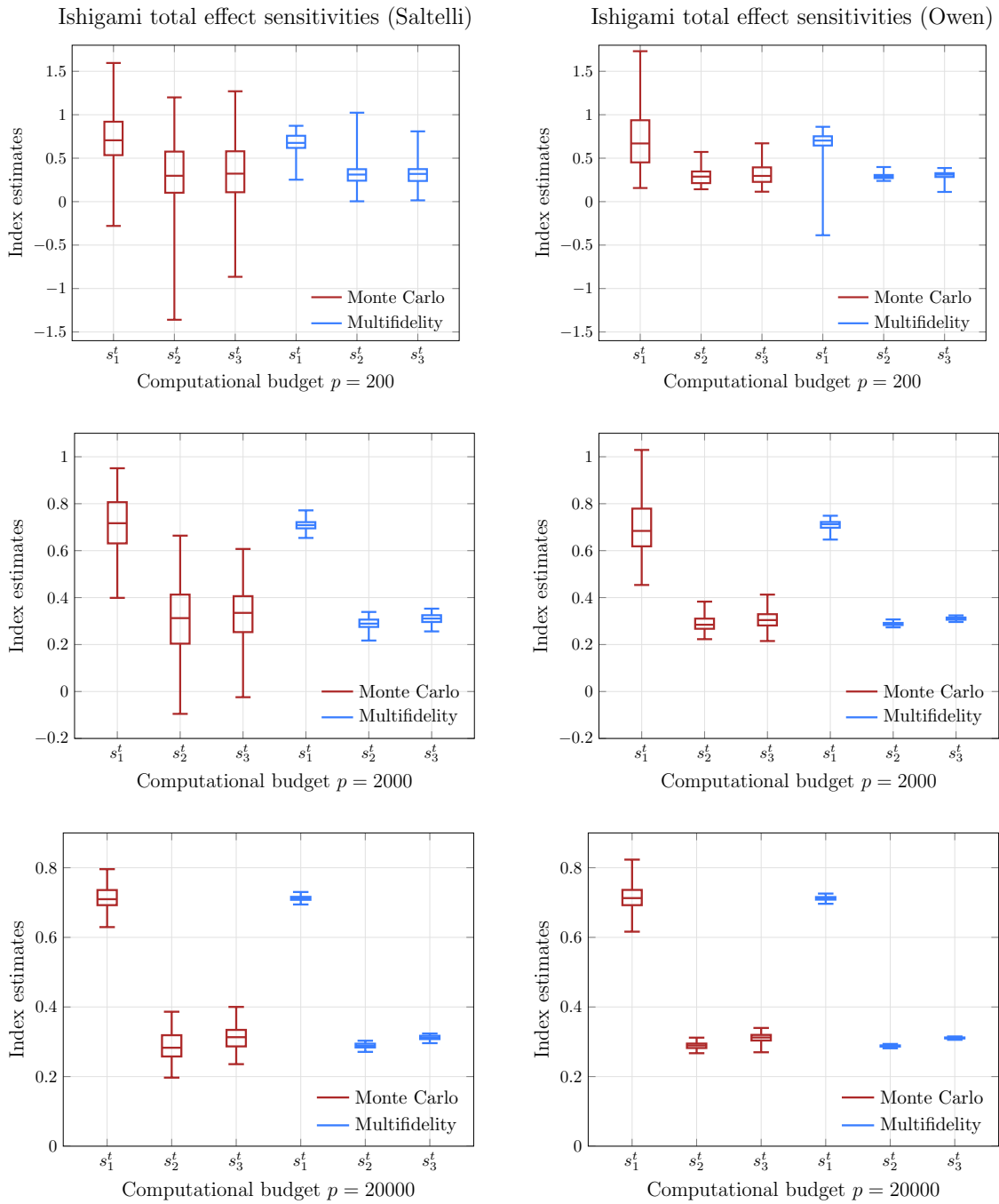
Figure 4: Comparison of multifidelity vs. Monte Carlo estimates of total effect sensitivities for the Ishigami function (21) with computational budgets p = 200, 2000, 20000 . Box plots are of one hundred estimator replicates. Left and right plots use the Saltelli and Owen estimators, respectively. Note that the Owen estimators outperform the Saltelli estimators on small sensitivity indices.
