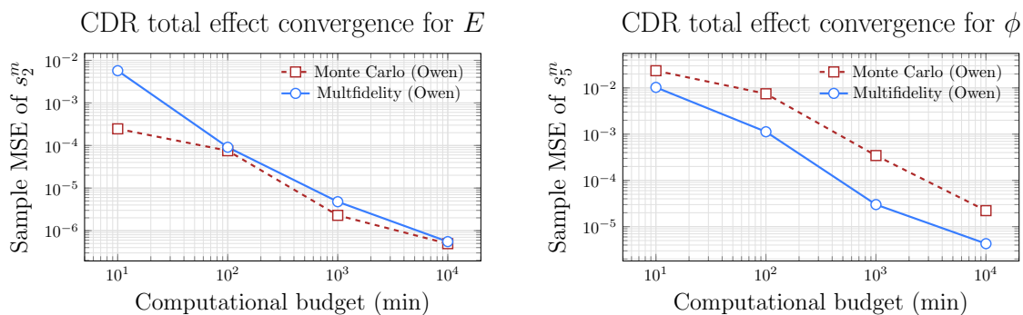
Figure 9: Sample MSEs of total sensitivity estimates using high-fidelity and multifidelity Monte Carlo. Results for one small (for E ) and one large (for \phi ) sensitivity are shown; the Owen estimators are so efficient that the multifidelity approach does not achieve efficiency gains for small sensitivity indices.
