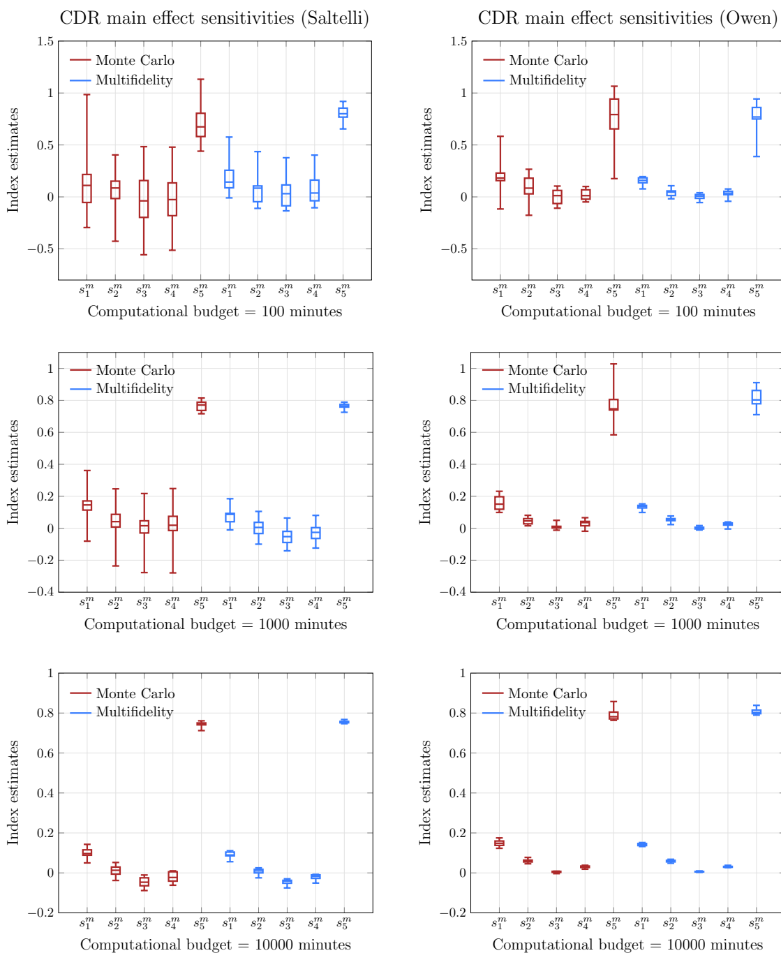
Figure 6: Box plots of one hundred main sensitivity index estimate replicates with vanilla Monte Carlo estimates in red and multifidelity estimates in blue. The multifidelity estimator outperforms the Monte Carlo estimator, and the Owen estimator outperforms the Saltelli estimator.
