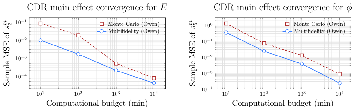
Figure 8: Sample mean-squared errors of main sensitivity estimates using high-fidelity and multifidelity Monte Carlo. Results for one small (for E ) and one large sensitivity (for \phi ) are shown.
