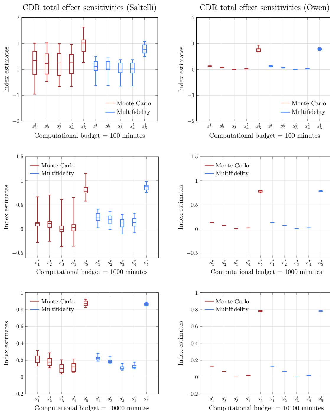
Figure 7: Box plots of one hundred total sensitivity index estimate replicates with vanilla Monte Carlo estimates in red and multifidelity estimates in blue. The Owen estimator significantly outperforms the Saltelli estimator. The multifidelity method outperforms a vanilla Monte Carlo approach for all Saltelli indices, but only achieves efficiency gains relative to the Owen estimator in the s_5^t estimate.
