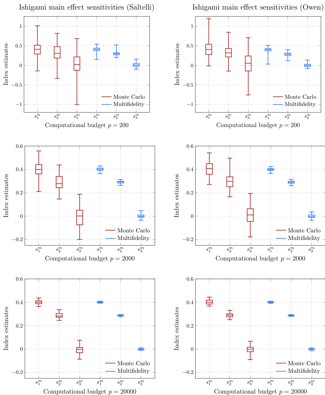
Figure 3: Comparison of multifidelity vs. Monte Carlo estimates of main effect sensitivities for the Ishigami function (21) with computational budgets p = 200, 2000, 20000 . Box plots are of one hundred estimator replicates. Left and right plots use the Saltelli and Owen estimators, respectively. The multifidelity estimators achieve desired accuracy faster than the MC estimators, allowing definitive ranking of inputs with p = 2000 , while Monte Carlo barely achieves this at p = 20000 .
