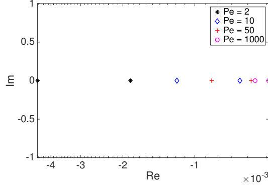
Figure 4: The two eigenvalues with largest real part of the system matrix A(q_i) from the convection-diffusion equation. The eigenvalues move closer to the imaginary axis as the Péclet number grows, and convection dominates.
