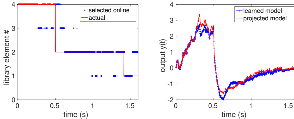
(a) Selected library elements as indicated by the detection function h(\cdot) for the convection-diffusion problem. (b) The output y(t) of the system with control derived from the updated model (+), compared to an “ideal” model where the matrices are known, and optimal controllers are available (—).
