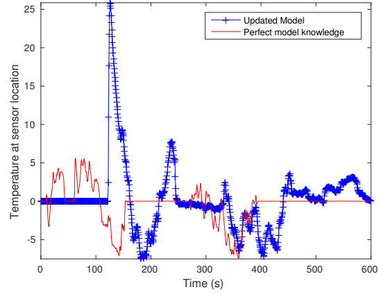
(b) The output y(t) of the system with control derived from the updated model (+), compared to an “ideal” model where the matrices are known, and optimal controllers are available (—)
