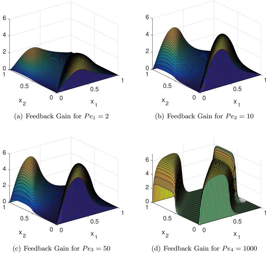
Figure 6: The feedback gains according to four different viscosities.
