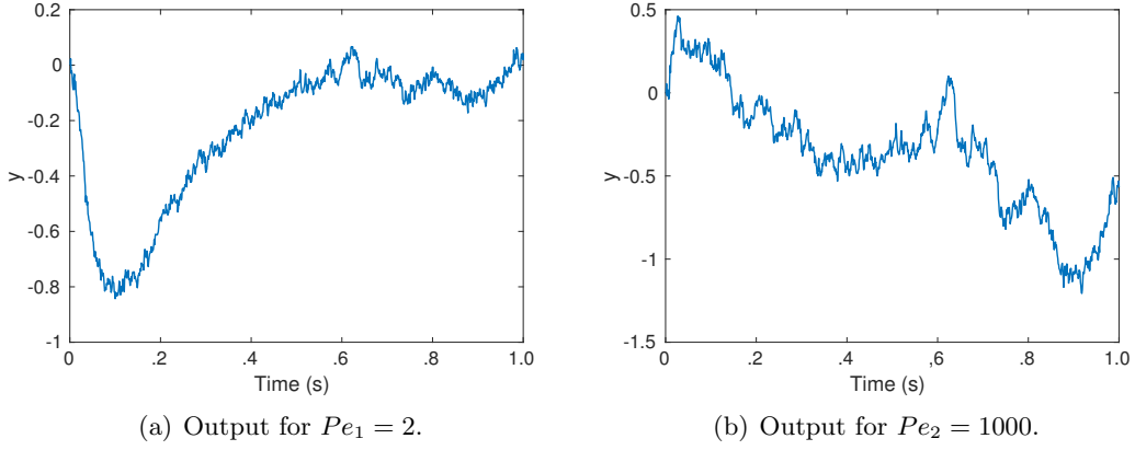
Figure 5: Output y(t) of the open loop convection diffusion system, excited with nonzero initial condition z_0 = 15 \sin(2\pi x) \sin(\pi y) and Gaussian disturbance g(t) with variance \sigma = 0.5 applied through a disturbance term at 0 \leq x_1 \leq 0.05 . For low Péclet number, the output returns to the zero state by the end of the simulation (a), whereas for high Péclet number the system remains away from the zero state (b).
