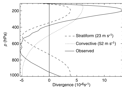
Figure 45. Divergence measured by rawinsondes when extensive, deep convection-generated cloud systems affected the intensive flux array (centered near 2^{\circ}\text{S} , 156^{\circ}\text{E} ) over the western tropical Pacific during TOGA COARE. Sixteen cases were used to compute the net divergence (solid curve). The components of the net divergence constituted by the 52 and 23 \text{ m s}^{-1} gravity wave responses to the mass disturbance are shown by the dotted and dashed curves, respectively. From Houze [1997], derived from calculations of Mapes and Houze [1995] and provided by B. Mapes, University of Colorado, Boulder.
