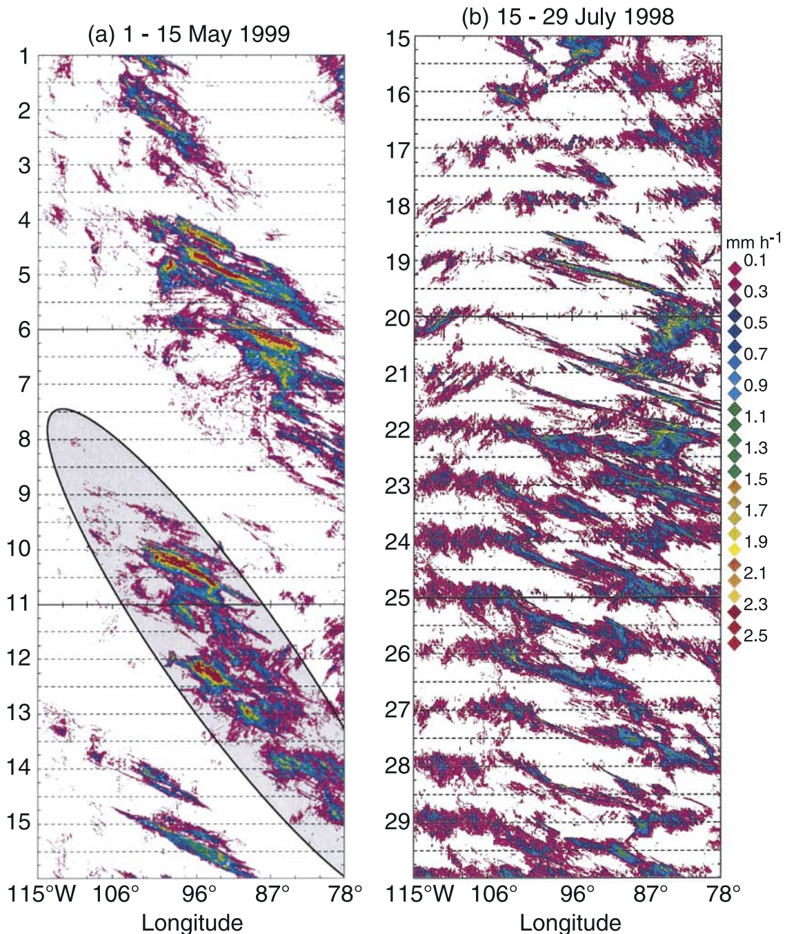
Figure 30. Time-longitude plot of radar-derived rain rate over the central United States for (a) 1–15 May 1999 and (b) 15–29 July 1998. Note the slow eastward propagation of precipitation envelopes in Figure 30a, within which there are faster propagating rain streaks. The shaded, elliptical area denotes one such envelope. In Figure 30b, there are mixed regimes including a nearly pure component of diurnal modulation in the western part of the domain. From Carbone et al. [2002].
