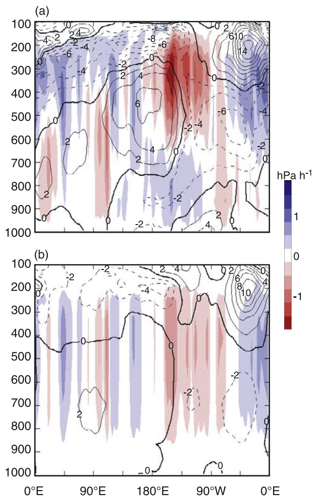
Figure 51. Vertical cross sections of anomaly fields of vertical motion (shaded) and zonal wind (contours dashed) averaged along the equator from 8.5^{\circ}\text{N} to 8.5^{\circ}\text{S} for the NCEP reanalysis basic state for El Niño (January, February, March, and April 1998) and latent heating derived from the TRMM PR-observed precipitation. (a) Observed, spatially variable stratiform rain fraction shown by the TRMM PR. (b) A stratiform rain fraction assumed to be a uniform 40% (the tropics-wide average). In this case the circulation is weak and without structure. The structure seen in the observed case (Figure 51a) derives from the spatial variability of the stratiform rain fraction. From Schumacher et al. [2004].
