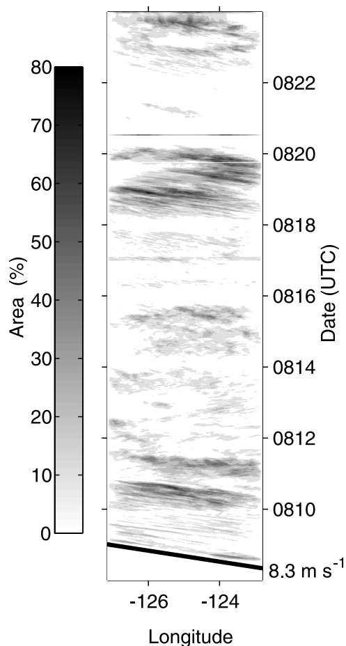
Figure 36. Time-longitude plot of ship radar data collected on 9–23 August 1997 at 7.8°N, 125°W in the middle of the east Pacific Intertropical Convergence Zone during the Tropical Eastern Pacific Process Study. Radar echo is represented as percent area covered by reflectivity >20 dBZ. The bold line indicates the easterly wave propagation speed of 8.3 \text{ m s}^{-1} as determined from satellite data. The streaks in the radar data indicate that the echoes tended to move at a similar zonal velocity. On 19 August these streaks were superimposed on an eastward propagating pattern, evidently associated with a Kelvin wave. From Serra and Houze [2002].
