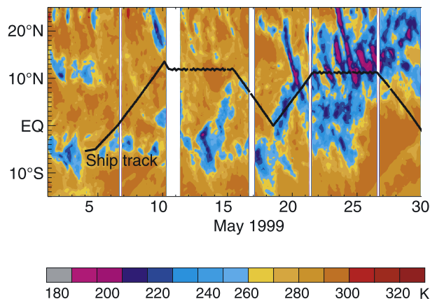
Figure 34. Time-latitude section of brightness temperature (see color-coded scale) from the European Space Agency METEOSAT-5 geostationary satellite. Data are averaged between 85° and 90°E. Cold temperatures are indicative of high cloud tops, while relatively clear periods appear as warm temperatures representing infrared radiation emitted at the surface or the moist boundary layer or from low tropospheric clouds. From Webster et al. [2002].
