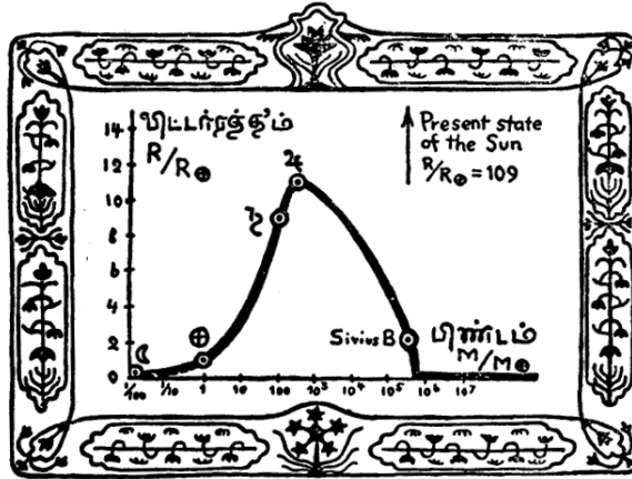
III. 62. The relationship between the radii and the masses of cold stellar bodies, according to the calculations of the Indian astrophysicist S. Chandrasekhar. The symbols \odot , \oplus , \otimes , and \otimes respectively represent the Moon, the Earth, Saturn, and Jupiter. Note that for masses greater than 460,000 times the mass of the Earth, the radius becomes zero! The words for mass and radius are in Dr. Chandrasekhar's original Tamil.
