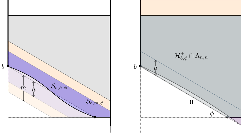
FIGURE 3. Left: the sets considered in Proposition 3.7, where we bound the probability of the interface exceeding height \pm h . Right: the proof of Lemma 3.8 uses monotonicity in b.c., to go from bounding the probability of the order-disorder interface exceeding height a in the gray set to the union of the gray and purple sets, to all shaded regions.
