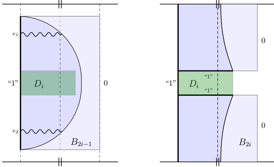
FIGURE 6. Left: the event \Gamma_{2i-1} where the interface of the component of \partial_W B_{2i-1} does not intersect D_i , and is connected to two edges e_1, e_2 that have no bridges. Right: the event \Gamma_{2i} where the interface of the component of \partial_W B_{2i} \cup \partial_{N,S} D_i does not intersect the dashed line. Overall, the intersection \Gamma_{2i-1} \cap \Gamma_{2i} pushes the interface forward by \ell n .
