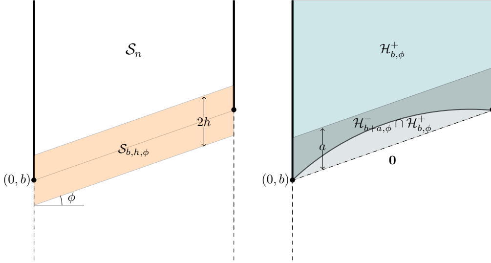
FIGURE 2. An illustration of some of the sets and interfaces considered in Definition 3.5 and Proposition 3.6. The (1, 0, \phi) boundary conditions are depicted with bold lines being wired and dashed lines being free.
