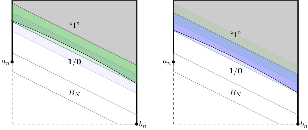
FIGURE 5. The green and blue blocks B_k, B_{k+1} are updated by the censored dynamics in two consecutive steps; with high probability, the chain (\bar{X}_{t_k}^0)_k pushes its interface down toward \langle a, b \rangle by \ell at every step, and is subsequently coupled to (\bar{X}_{t_k}^1)_k on the growing gray region.
