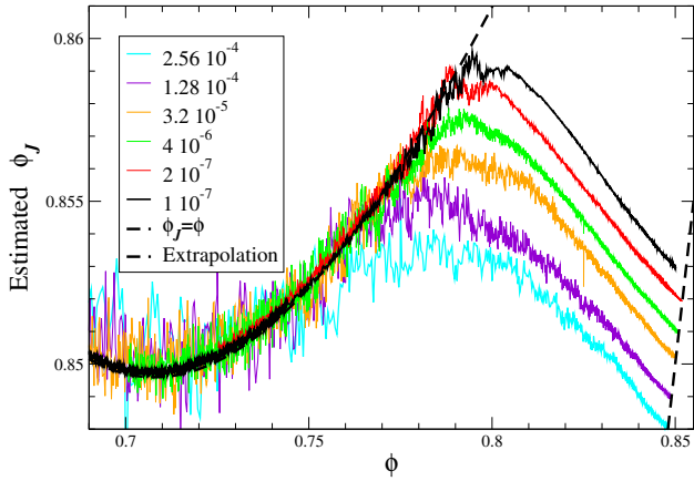
Figure 1: The equation of state \tilde{\phi}_J(\phi) for N = 4096 disks as observed by compressing a liquid with different expansion rates \gamma (see legend).
