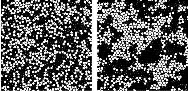
Figure 4: The microstructure of a packing without (left, \phi_J \approx 0.846 ) and with moderate clustering (right, \phi_J \approx 0.850 ).
