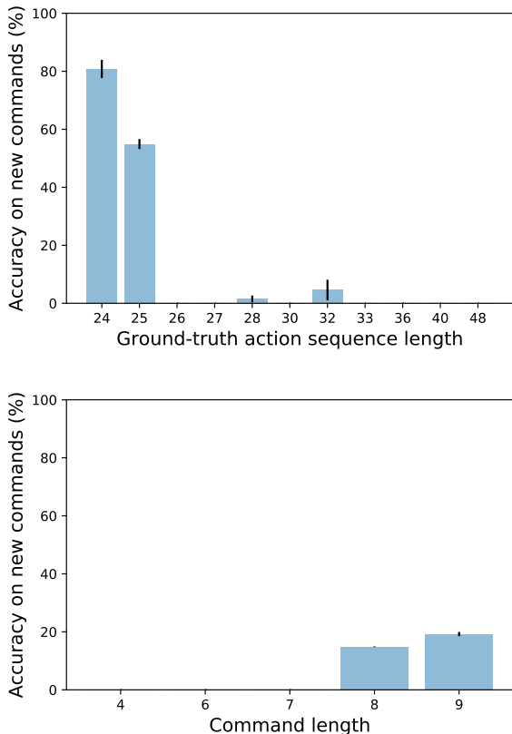
Figure 4. Zero-shot generalization to commands with action sequence lengths not seen in training. Top: accuracy distribution by action sequence length. Bottom: accuracy distribution by command length (only lengths attested in the test set shown, in both cases). Bars show means over 5 runs of overall-best model with \pm 1 SEM.
