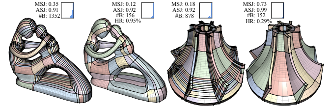
Fig. 10. Simplified results (right) on meshes (left) generated with the frame-field based method [Li et al. 2012].
