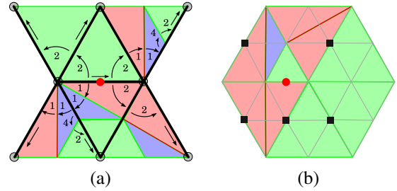
Figure 4: (a) Some triangles in the stencil have been refined beyond the level of the splitting edge. (b) Some triangles in the stencil are at a level lower than that of the splitting edge (marked with a red bullet).
