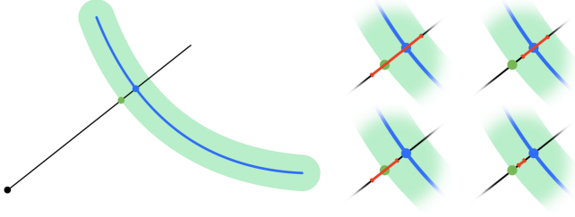
Fig. 3. An \varepsilon, \delta -MINIMIZE Problem: the first intersection between the black segment and the blue line is sought. The segment starts at the black bullet. The blue bullet corresponds to solution F^* of the corresponding Minimization Problem in the continuum. The green bullet corresponds to the solution for region \Phi_\varepsilon , whose image is the green area. The red segments in the blow-ups to the right correspond to possible intervals \tilde{F}^* returned as numerical solutions. Their lower ends are guaranteed to lie below the blue bullet and their upper ends are guaranteed to lie beyond the green bullet. The different configurations arise from the interplay between the values of \varepsilon and \delta : as \varepsilon tends to zero, the upper left configuration becomes more frequent; as \delta tends to zero, the lower right configuration becomes more frequent.
