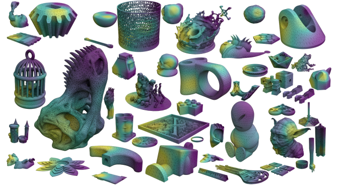
Fig. 14. Sample models from our optimized 3D dataset composed of 9809 tetrahedral meshes generated with TetWild [Hu et al. 2018] using default parameters, the colors represent the Dirichlet boundary conditions used to solve the Poisson problem on the interior.
