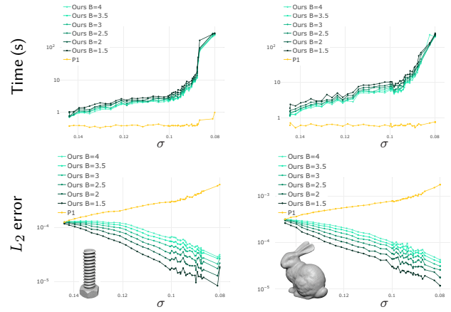
Fig. 9. Poisson solutions on a series of remeshing of the same boundary mesh with varying quality (measured by the shape parameter \sigma , x-axis). Plot of the running times in seconds (top) and L_2 errors (bottom) for different choices of B .
