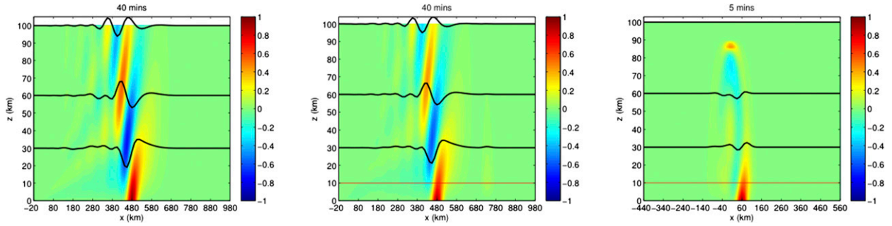
FIG. 5. As in Fig. 1, but for the compressible model. (left) Uniform stratification at t = 40 min; (middle) with tropopause; (right) with tropopause at t = 5 min, showing a fast acoustic precursor wave that is clearly absent in Fig. 1.
