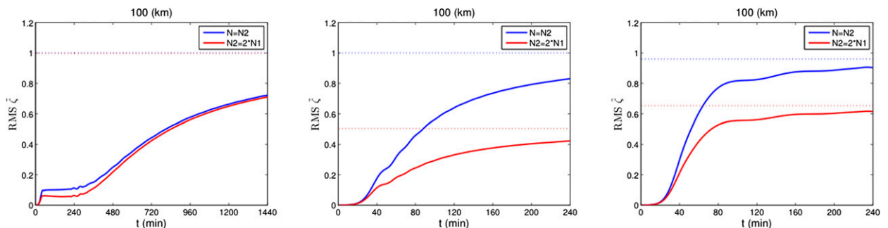
FIG. 2. Time evolution of anelastic gravity wave amplitudes at z = 100 \text{ km} with a tropopause (red line) and without (blue line). The tsunami speeds across the panels are (left) V = 30 , (middle) V = 100 , and (right) V = 200 \text{ m s}^{-1} ; and the stippled lines indicate the asymptotic steady-state limit; note the much longer integration time for V = 30 \text{ m s}^{-1} . In the V = 200 \text{ m s}^{-1} case, the uniformly stratified limit is less than unity, because part of the wave field is evanescent.
