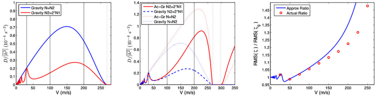
FIG. 3. (left) Pseudomomentum flux D as a function of V in anelastic model with and without a tropopause. (middle) Pseudomomentum flux D for larger range of V and for both anelastic and compressible models with and without a tropopause. The forbidden tsunami speed zone is clearly visible. (right) Root-mean-square ratio of acoustic-gravity waves to anelastic gravity waves in case with tropopause. The red circles are the actual ratios, and the blue solid line is the scaled pseudomomentum flux ratio \sqrt{\beta^2 D/D_g} , which crudely measures the increased back-reflection in the anelastic case. Without a tropopause, this scaled pseudomomentum flux ratio would be unity by (33).
