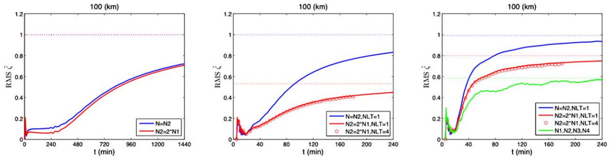
FIG. 4. As in Fig. 2, but for compressible acoustic gravity waves. In the first 5–10 min, a signal due to a fast acoustic precursor wave is clearly visible. The plots also indicate that our results are insensitive to the value of the number of tropospheric layers used in the numerical model (NLT), see section 3c. The blue dotted lines indicate the asymptotic steady-state limit of the isothermal fully compressible model, in agreement with the one proposed by Peltier and Hines (1976). Compared to Fig. 2, the evanescent part of the compressible wave field is much weaker at V = 200 \text{ m s}^{-1} , and hence the asymptotic amplitude in the uniformly stratified case is almost unity. (right) The green lines are the solutions with a more realistic atmospheric profile summarized in Table 1. This solution is qualitatively similar to the one plotted in red lines, but with a smaller amplitude, due mostly to partial reflection around the mesopause and to the larger rigidity (i.e., smaller density scale height H ) above the mesosphere.
