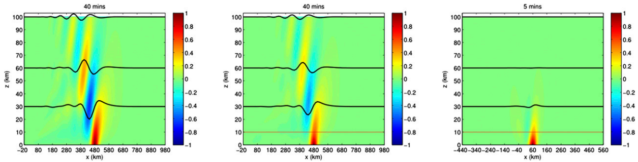
FIG. 1. Snapshots of scaled vertical displacement \tilde{\zeta} in the anelastic model for V = 200 \text{ m s}^{-1} . Also shown are three line plots defined by z + 15000 \times \tilde{\zeta}(x, z, t) , with z \in \{30, 60, 100\} \text{ km} , respectively. These are material lines with greatly exaggerated deformations, and they illustrate that shorter scales travel faster than longer scales. (left) Uniform stratification at t = 40 \text{ min} ; (middle) with tropopause located at z = 10 \text{ km} ; (right) with tropopause, but at earlier time t = 5 \text{ min} .
