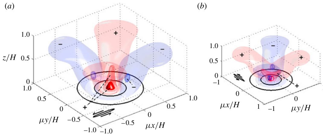
FIGURE 5. (Colour online) (a) As figure 3(b) but for \gamma = 0.1 . The two outermost isocontours correspond to the same values as in figure 3, whereas the innermost isocontour corresponds to C_x^L/(aU_0\omega) = 4 \times 10^{-6} ( \max[C_x^L/(aU_0\omega)] \approx 5.0 \times 10^{-6} ). The tidal double arrow of figure 3 has turned into a counterclockwise tidal ellipse of aspect ratio \gamma . (b) As (a) but with viewpoint rotated by 90^\circ in the horizontal.
