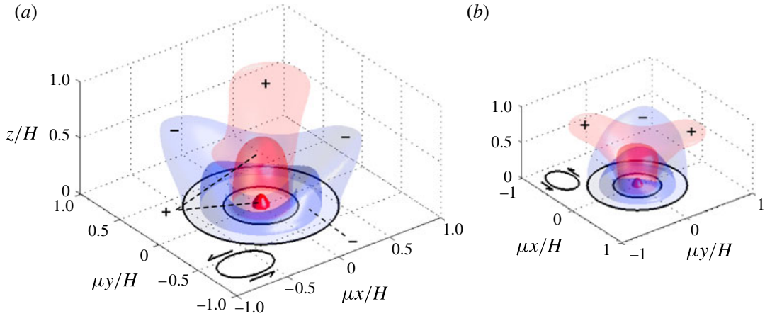
FIGURE 6. (Colour online) As figure 5 but for \gamma = 0.7 , and the innermost isocontour now corresponds to C_z L / (aU_0\omega) = 30 \times 10^{-6} ( \max[C_z L / (aU_0\omega)] \approx 35 \times 10^{-6} ).
