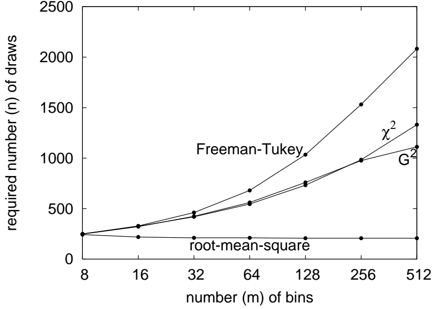
Figure 25: Seventh example; see Subsection 5.2.7.
