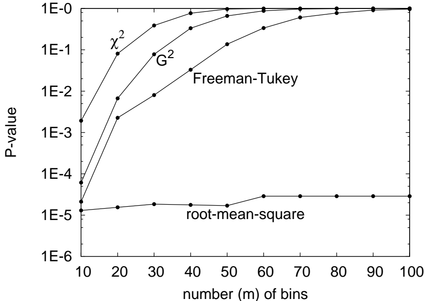
Figure 1: P-values for the hypothesis that the model (10)–(12) agrees with the data of 15 draws in the first bin, 5 draws in the second bin, and no draw in any other bin
