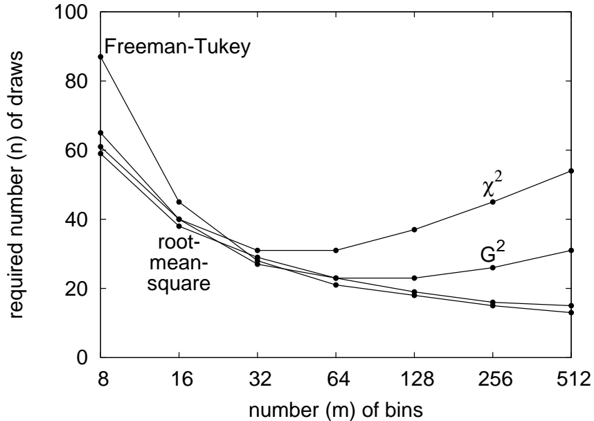
Figure 24: Sixth example; see Subsection 5.2.6.
