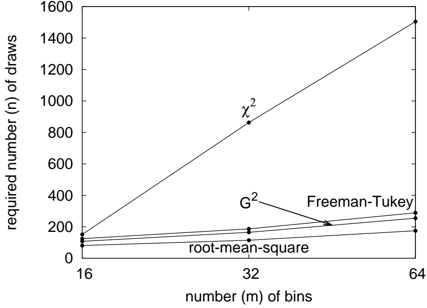
Figure 17: Sixth example; see Subsection 5.1.6.
