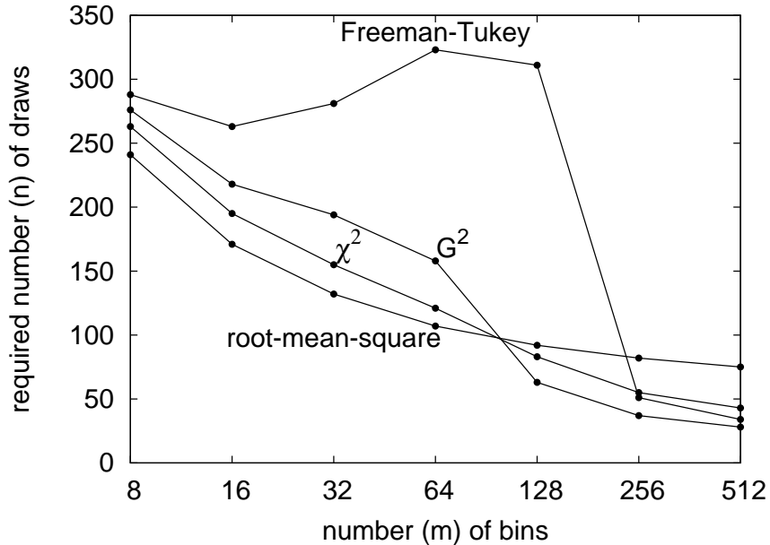
Figure 14: Third example; see Subsection 5.1.3.
