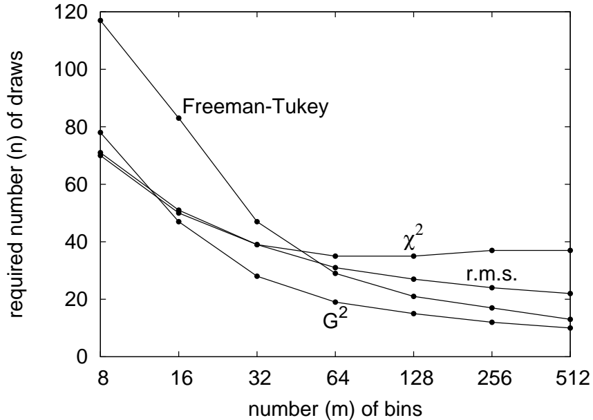
Figure 16: Fifth example; see Subsection 5.1.5.
