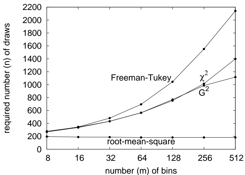
Figure 12: First example (statistical “efficiency”); see Subsection 5.1.1.
