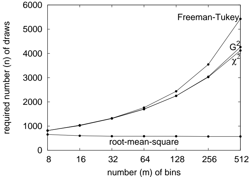
Figure 22: Fourth example; see Subsection 5.2.4.
