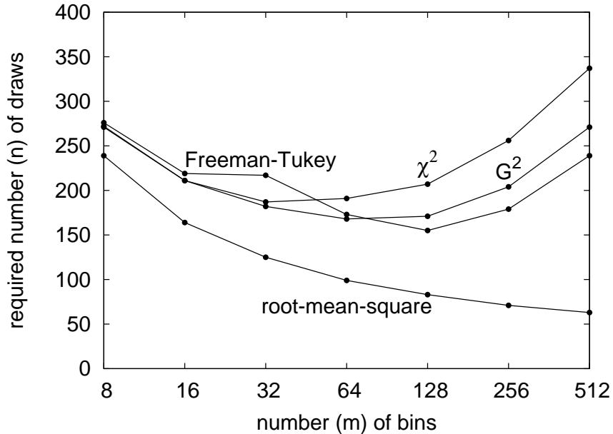
Figure 15: Fourth example; see Subsection 5.1.4.
