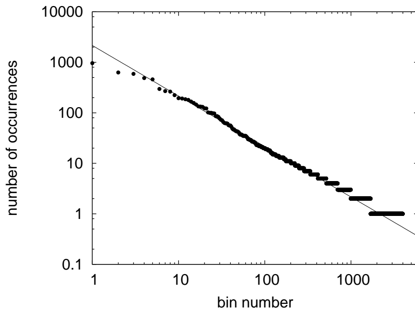
Figure 5: Numbers of occurrences of the various words (one bin for each distinct word) in a corpus of 20,000 random draws from List 5 of Eldridge (2010)
