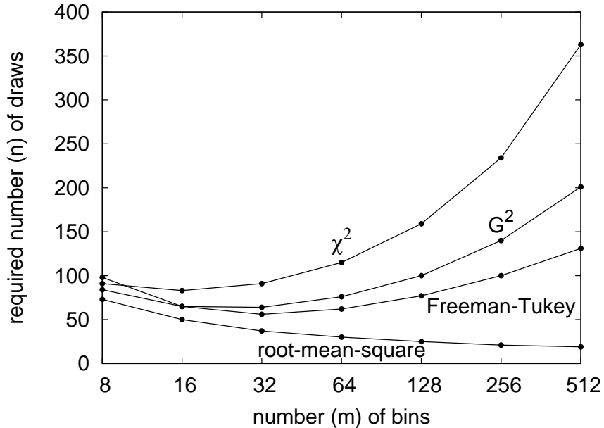
Figure 13: Second example; see Subsection 5.1.2.
