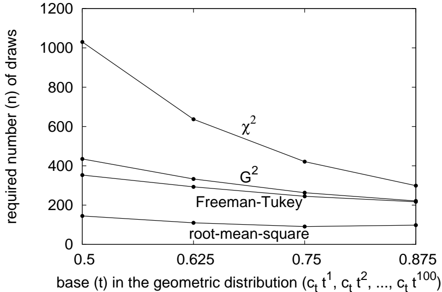
Figure 19: First example; see Subsection 5.2.1.
