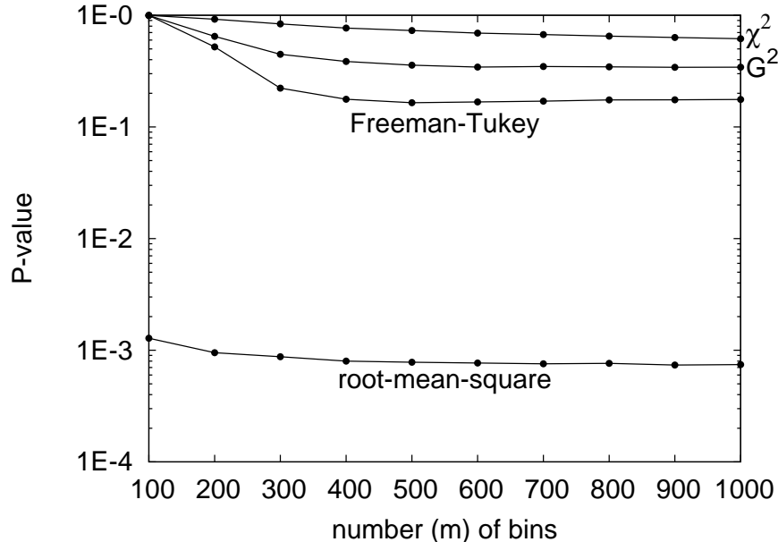
Figure 2: P-values for the hypothesis that the model (10)–(12) agrees with the data of 36 draws in the first bin, 12 draws in the second bin, 1 draw each in bins 3, 4, \dots , 50, and no draw in any other bin
