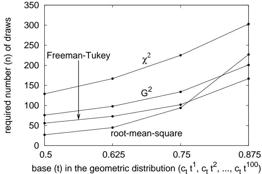
Figure 18: Seventh example; see Subsection 5.1.7.
