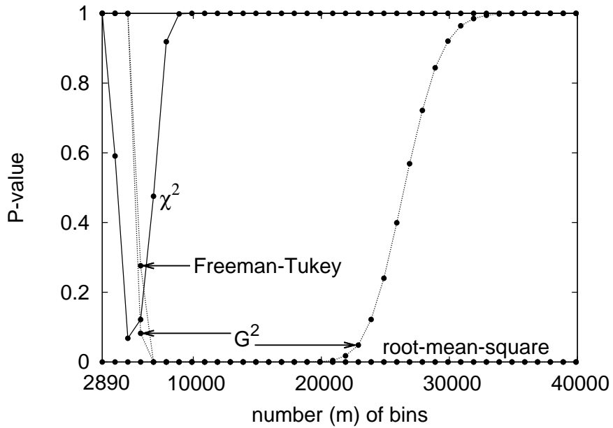
Figure 4: P-values for the data plotted in Figure 3 to follow the Zipf distribution
