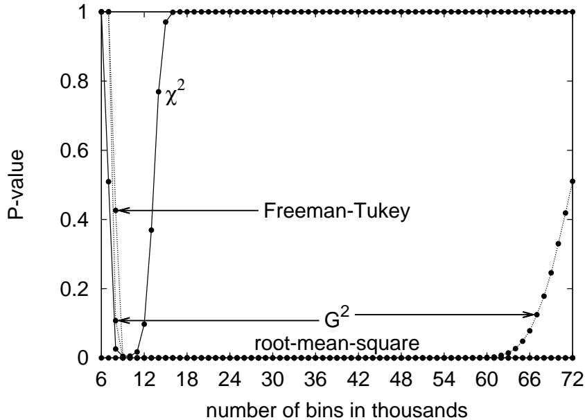
Figure 6: P-values for the data plotted in Figure 5 to follow the Zipf distribution
