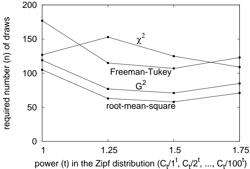
Figure 20: Second example; see Subsection 5.2.2.
