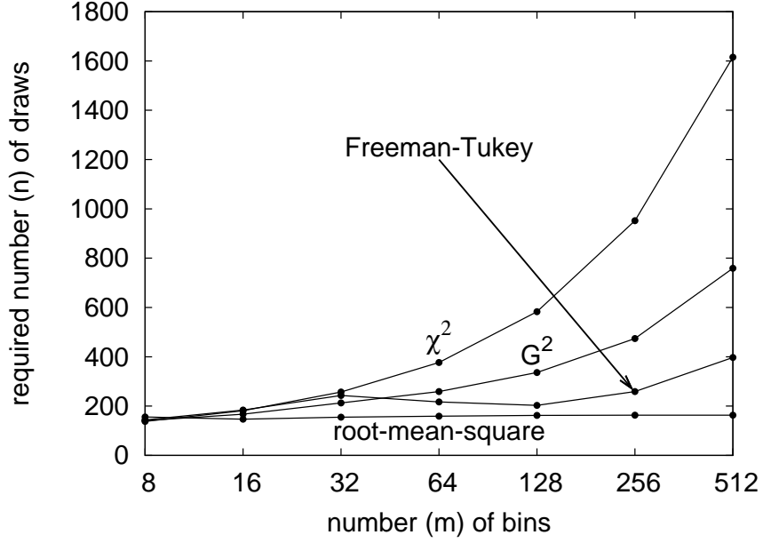
Figure 23: Fifth example; see Subsection 5.2.5.
