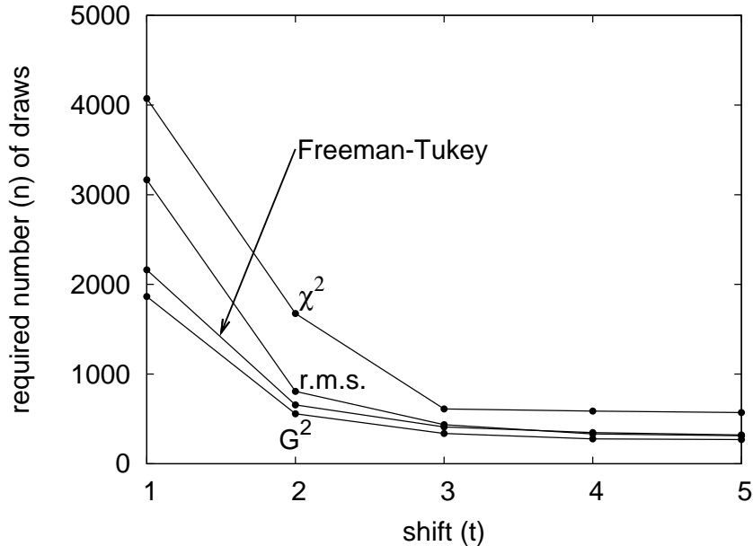
Figure 21: Third example; see Subsection 5.2.3.
