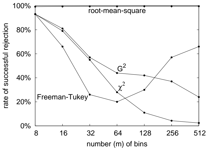
Figure 11: First example, with n = 200 draws; see Subsection 5.1.1.
