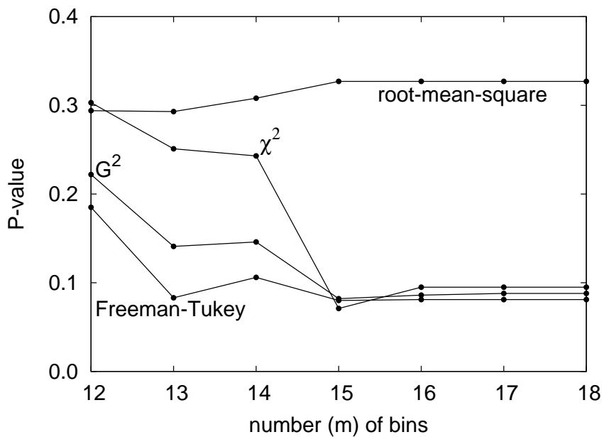
Figure 8: P-values for the distribution of Table 1 to be Poisson
