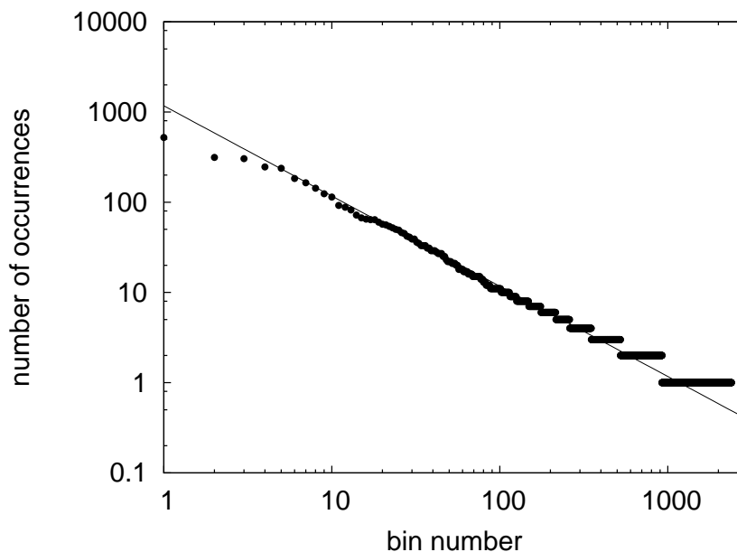
Figure 3: Numbers of occurrences of the various words (one bin for each distinct word) in a corpus of 10,000 random draws from List 1 of Eldridge (2010)
