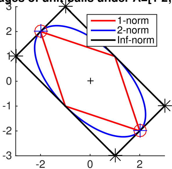
Images of unit-balls under A=[1 \ 2; 1 \ -2]
