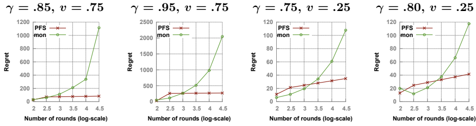
Figure 2: Comparison of the monotone algorithm and \text{PFS}_r for different choices of \gamma and v . The regret of each algorithm is plotted as a function of the number rounds when \gamma is not known to the algorithms (first two figures) and when its value is made accessible to the algorithms (last two figures).
