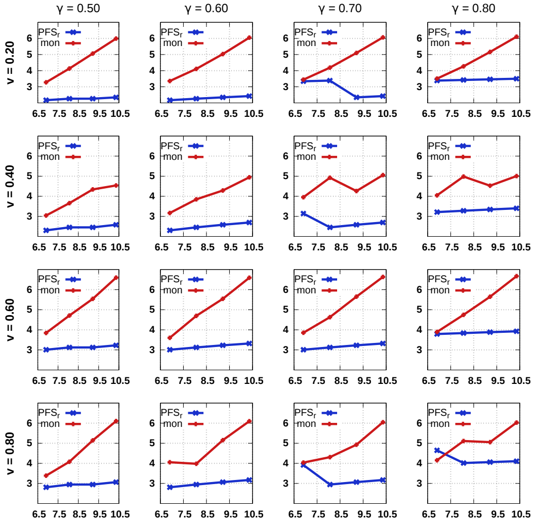
Figure 4: Regret curves for PFS_r and mon for different values of v and \gamma . The value of \gamma is known to both algorithms.
