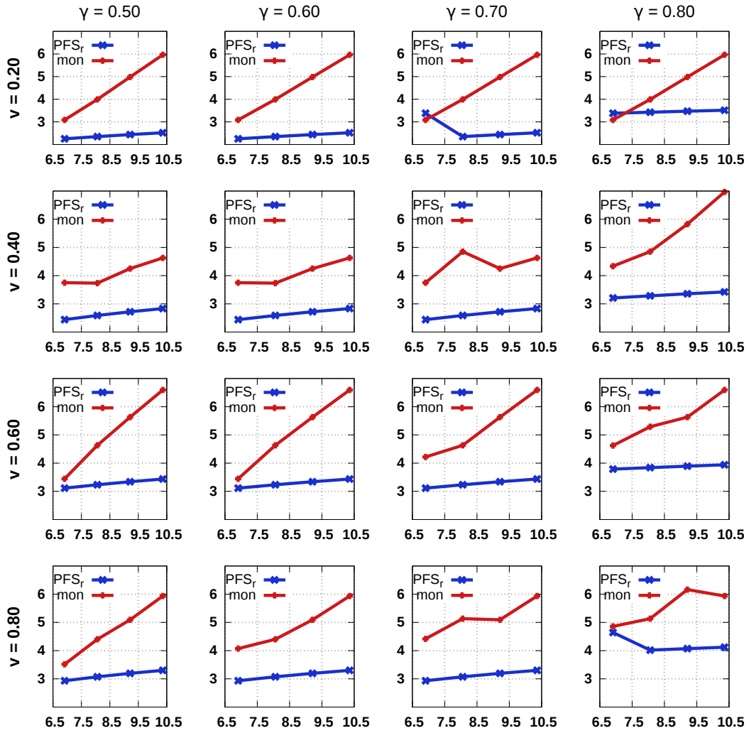
Figure 3: Regret curves for PFS_r and mon for different values of v and \gamma . The value of \gamma is not known to the algorithms.
