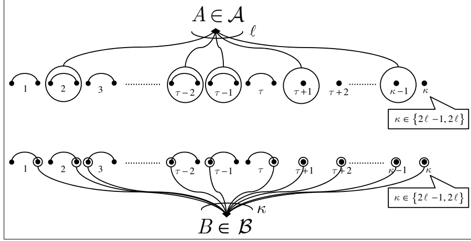
Figure 1: The extremal family (5) of \ell -cross-intersecting pairs \mathcal{A}, \mathcal{B} in case n = \kappa + \tau .
