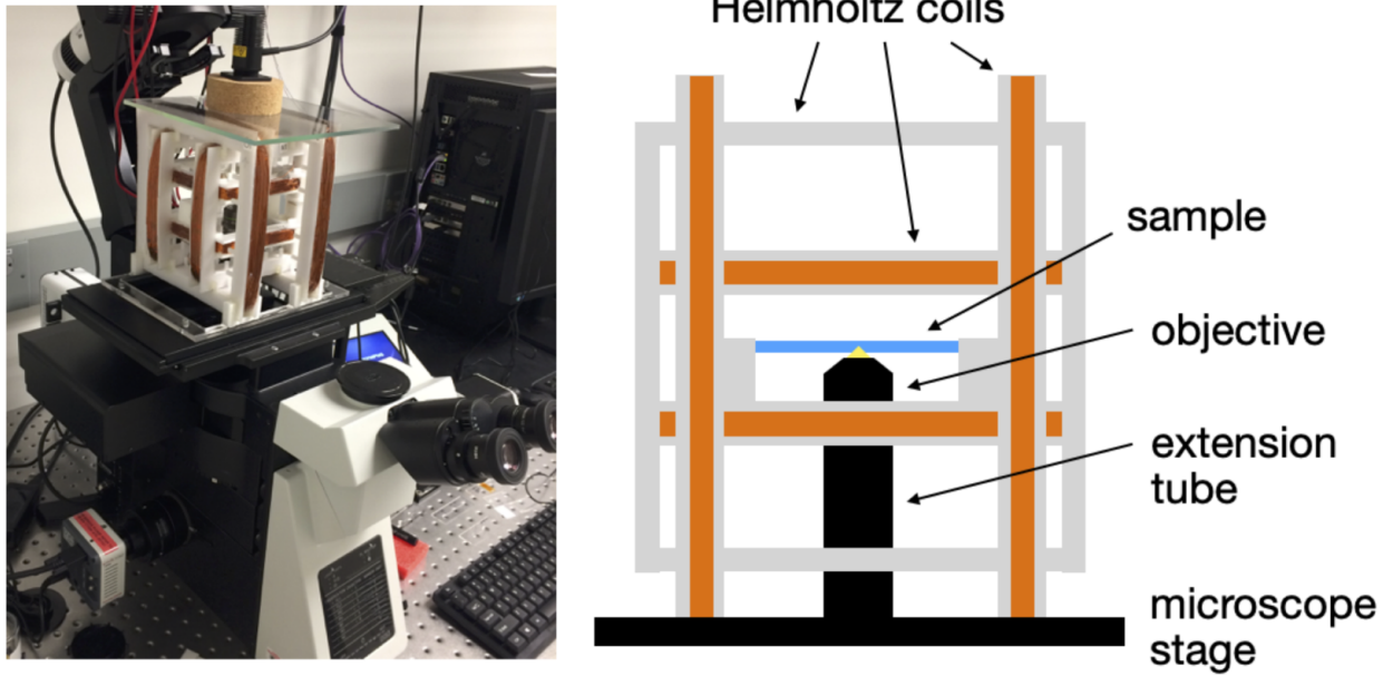
Figure 10: Photograph and schematic (side view) of the setup used for the roller experiments. The setup consists of a home-built tri-axial Helmholtz coil set [41] mounted on the stage of an inverted microscope. The sample is placed in the center of the coil set and the microscope objective is raised into the coil set using an extension tube.
