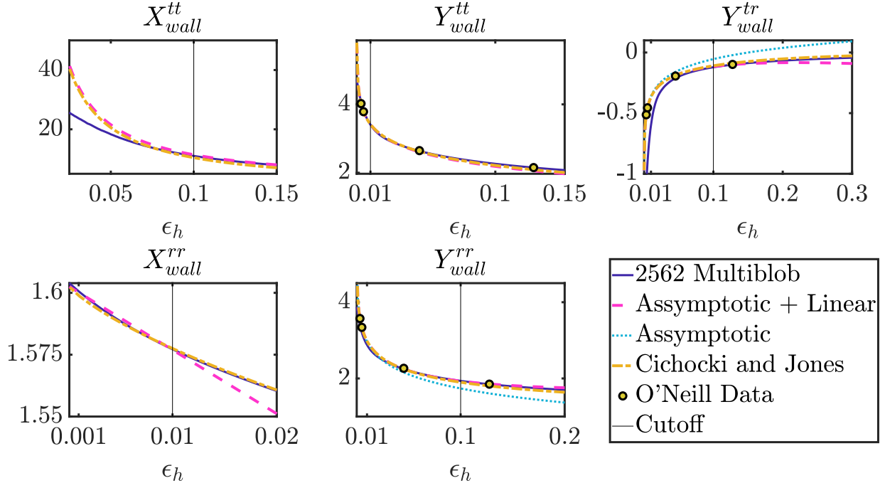
Figure 6: Coefficients of \mathcal{R}_{\text{lub}}^{\text{wall}} appearing in equation (7) as a function the normalized gap \epsilon_h . Each panels shows that value of one of the coefficients computed using the rigid multiblob method [31] with 2562 blobs (solid blue line), and the corresponding asymptotic result from table I (dashed pink line). Plots for Y_{\text{wall}}^{tr} and Y_{\text{wall}}^{rr} include the original asymptotic results computed in [4] (dotted green line) as well as our modification to include a linear term (where appropriate). The 9/9 Padé approximation given by Cichocki and Jones [27] (dot-dashed yellow line) agrees well with out ‘Asymptotic+Linear’ results within the cutoff regions. Plots for Y_{\text{wall}}^{tt} , Y_{\text{wall}}^{tr} , and Y_{\text{wall}}^{rr} also show data calculated by O’Neill (circles) and compiled in tables 1.1 and 2 respectively in [4]. The vertical black lines show the cutoff transitions between different estimates.
