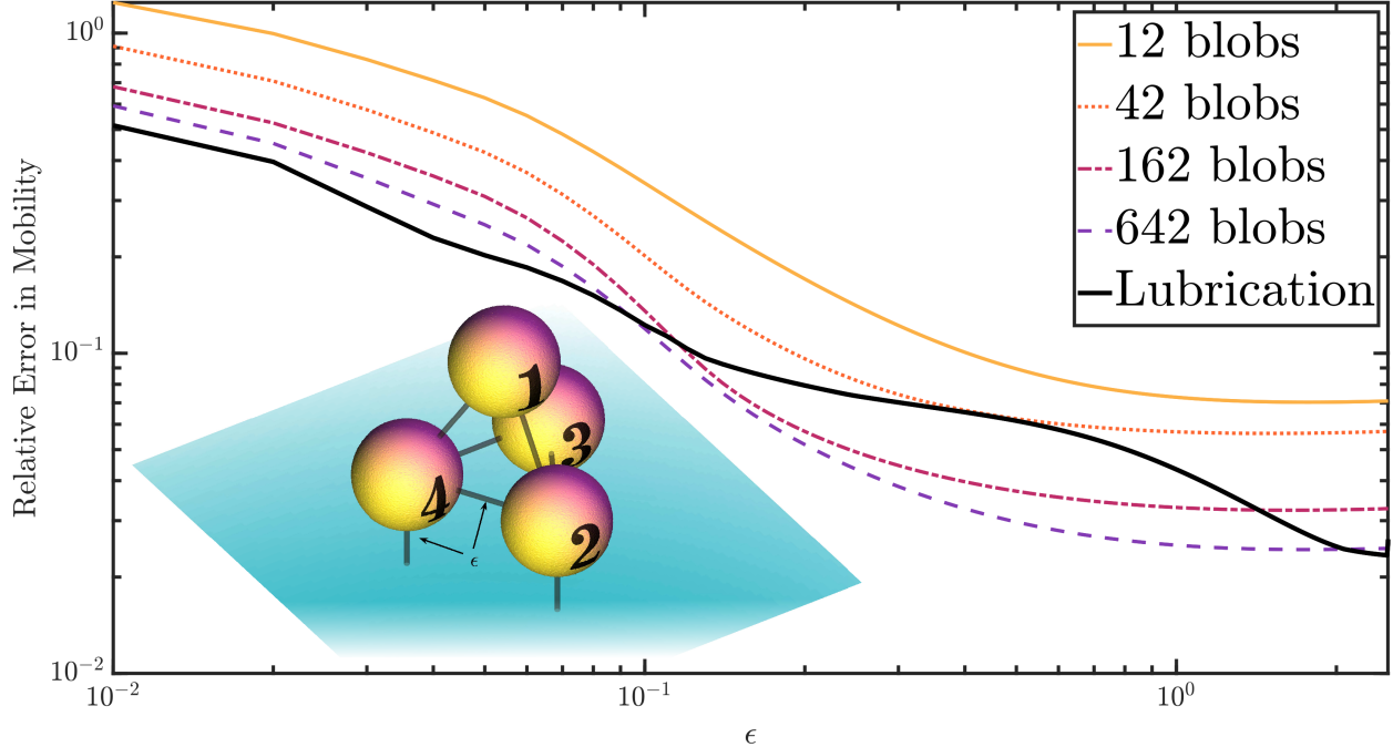
Figure 7: Relative L_2 error in the mobility matrix of the colloidal tetrahedron shown in the inset as a function of the relative gap \epsilon , for the lubrication-corrected mobility \overline{\mathcal{M}} (solid black line), as well as the mobility matrix computed using the rigid multiblob method [31] using 12, 42, 162, and 642 blobs to discretize each sphere. The error is measured relative to the mobility matrix computed using 2562 blobs to discretize each sphere.
