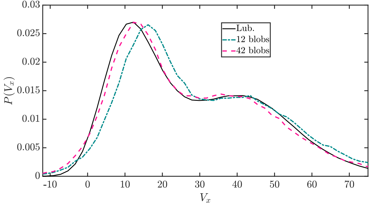
Figure 8: Histogram of one-step velocities for a dense uniform suspension of microrollers, computed using the lubrication-corrected STS scheme developed here (solid line), and the TS scheme of [3] using 12 (dashed-dotted) and 42 (dashed) blobs to discretize each sphere in the suspension.
