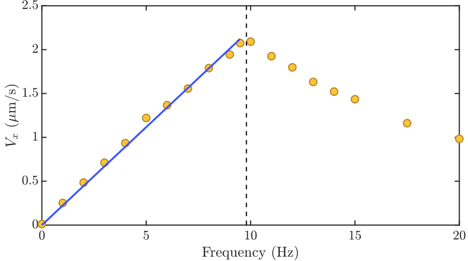
Figure 1: Measured velocity of dilute microrollers as a function of the frequency of the applied rotating magnetic field (40 G). Up to a frequency of \sim 9.8 Hz (vertical black dashed line), the velocity increases linearly with the frequency (blue line, slope = \bar{A}_f = 0.223 \mu\text{m} ). At higher frequencies the velocity decreases for increasing frequency, as the rollers cannot overcome the viscous torque of the surrounding liquid.
