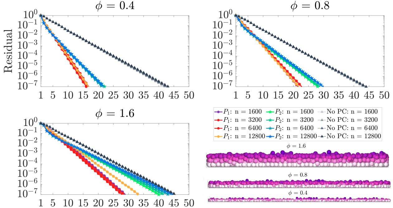
Figure 9: Convergence rates of the GMRES solver for (10) using the proposed preconditioner \mathbf{P}_1 , the block diagonal preconditioner \mathbf{P}_2 [10], as well as an unpreconditioned GMRES method for reference (termed ‘No PC’ in the legend). Each panel shows convergence rates for a fixed value of \phi , as the number of particles N_p is varied. Below the legend is a frontal view of the particle configurations for N_p = 3200 and for each value of \phi . Particles are colored based on their height above the wall with the highest particles colored the darkest while the lowest particles are colored the lightest. Higher values of \phi cause multiple layers of particles to form.
