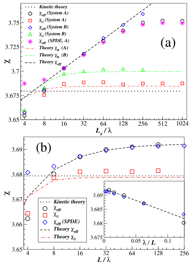
Figure 2: (Color online) (Panel a) The effective \chi_{\text{eff}} and the renormalized \chi_0 diffusion coefficients as a function of the width of the system L_x in two dimensions. Numerical results for System A (DSMC and SPDE) and System B (DSMC) are shown with symbols (see legend). The error bars for all of the simulation data are comparable or smaller than the size of the symbols. The theoretical predictions [12] are evaluated numerically and shown with lines. (Panel b) Same as panel (a) but in three dimensions. The inset highlights the L^{-1} behavior.
