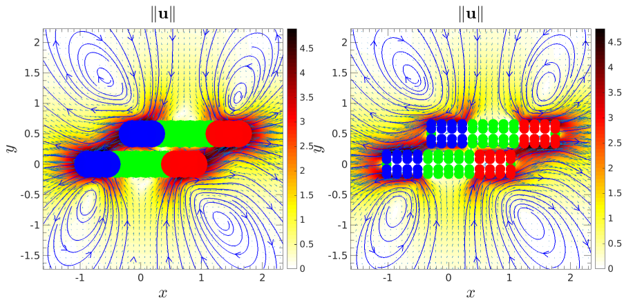
Figure : Active flow around a pair of extensile three-segment nanorods (Au-Pt-Au) sedimented on top of a no-slip boundary (the plane of the image) and viewed from above. The dimers are rotating together at \approx 0.7\text{Hz} in the counter-clockwise direction, consistent with recent experimental observations.
