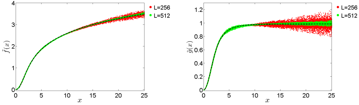
Figure 15: Empirical fits (lines) to numerical data (symbols) for \tilde{f}(x) (left) and \tilde{g}(x) (right), for the 6-point kernel in two dimensions, obtained using a periodic system of either 256^2 or 512^2 grid cells. Observe that both follow the correct asymptotic behavior at large distances, with scatter dominated by boundary effects.
