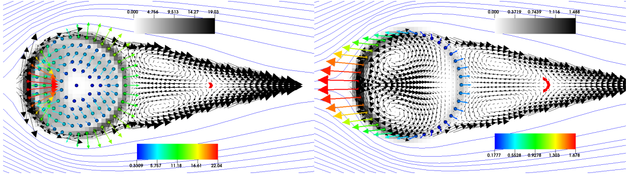
Figure 12: Steady incompressible flow at \text{Re} = 10 past a periodic column of cylinders represented as either filled disks of 121 markers (left) or a shell of 39 markers (right). We show the magnitude of the Eulerian constraint force \mathcal{S}\mathbf{\Lambda} (gray color map), the streamlines outside of the wake (solid blue lines), the wake velocity field (black arrows), and the Lagrangian constraint forces associated with each marker (color arrows). The red arrow marks the stagnation point where v_x = 0 , as used to determine the wake length.
