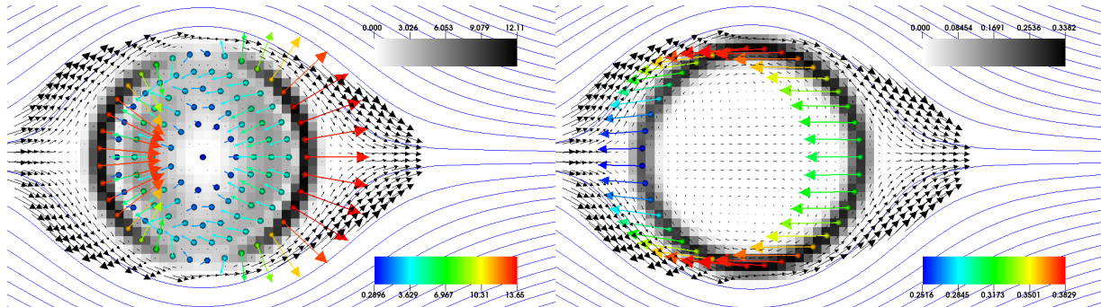
Figure 1: Two-dimensional Steady Stokes flow past a periodic column of circular cylinders (disks) at zero Reynolds number obtained using our rigid-body IB method (the same setup is also studied at finite Reynolds numbers in Section VII F). The markers used to mediate the fluid-body interaction are shown as small colored circles. The Lagrangian constraint forces \mathbf{\Lambda} that keep the markers at their fixed locations are shown as colored vectors; the color of the vectors and the corresponding marker i are based on the magnitude of the constraint force \mathbf{\Lambda}_i (see color bar). The fluid velocity field is shown as a vector field (black arrows) in the vicinity and the interior of the body; further from the body, flow streamlines are shown as solid blue lines. The magnitude of the Eulerian constraint force \mathbf{S}\mathbf{\Lambda} is shown as a gray color plot (see greyscale bar). (Left panel) A volume marker grid of 121 markers is used to discretize the disk. The majority of the constraint forces are seen to act near the surface of the body, but nontrivial constraint forces are seen also in the interior of the body. (Right panel) A surface grid of 39 markers is used to discretize the disk, which strictly localizes the constraint forces to the surface of the body.
