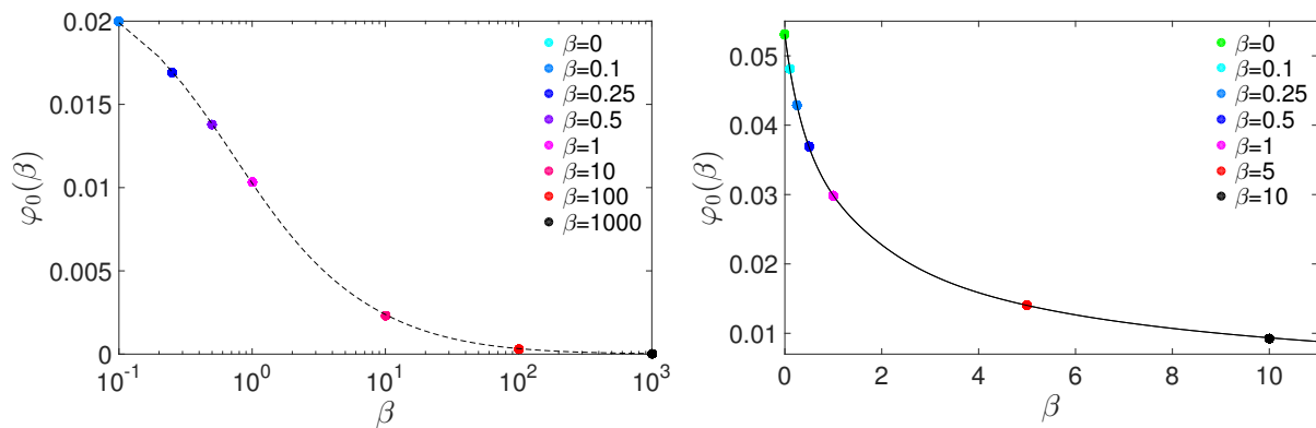
Figure 16: Empirical fit for \varphi_0(\beta) as a function of \beta for different values of \beta . (Left) Three dimensions, 256^3 grid. (Right) Two dimensions, 512^2 grid.
