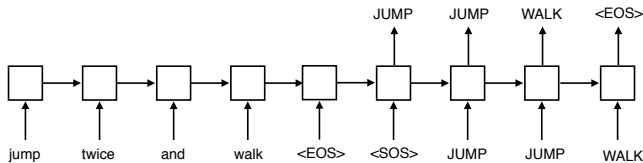
Figure 2. The seq2seq framework is applied to SCAN. The symbols <EOS> and <SOS> denote end-of-sentence and start-of-sentence, respectively. The encoder (left) ends with the first <EOS> symbol, and the decoder (right) begins with <SOS>.
